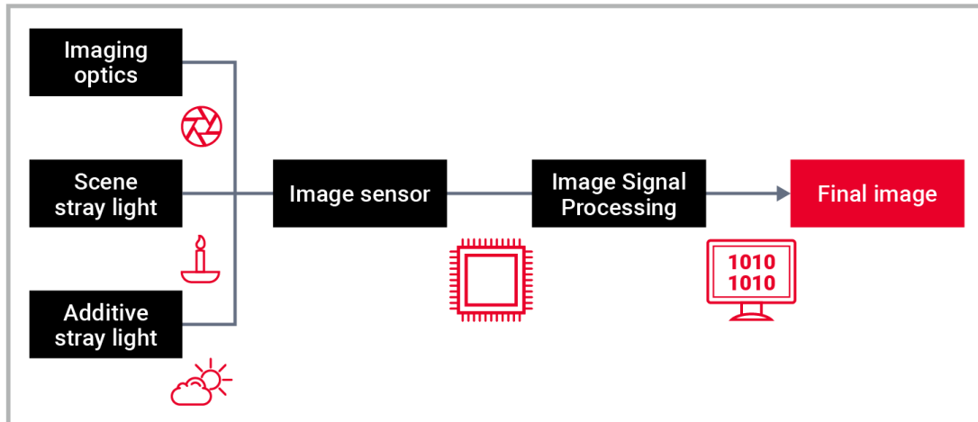
Figure 3. The simulated image from the imaging optics is combined with stray light effects from the scene and from an external source, and the combined irradiance is processed by the image sensor model and post processed using built-in or custom Image Signal Processing routines
