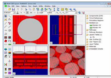
RSoft CAD Environment
